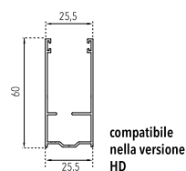
Guida in alluminio A60 25,5X60 mm
